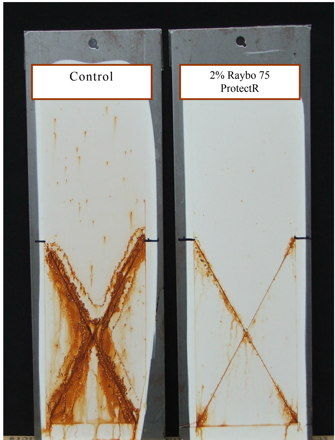
96 Hrs. Salt Spray - Cold Rolled Steel Q Panels
